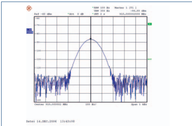
IM plot with electrolytic nickel as barrier layer
