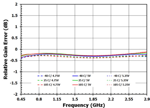
Figure 26. Relative Gain Error, DSA2 = 10dB, Bypass OFF
