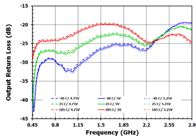
Figure 80. S22, DSA3 = 12dB, Bypass OFF
