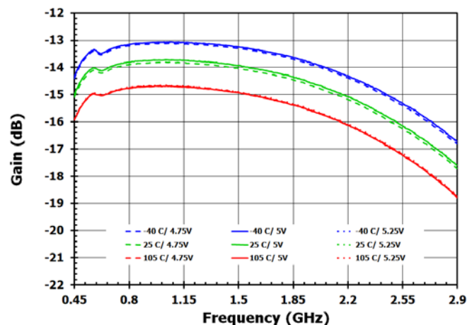
Figure 18. Gain, DSA3 = 6dB, Bypass ON
