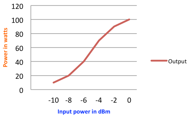
Output Power vs. Input Power
