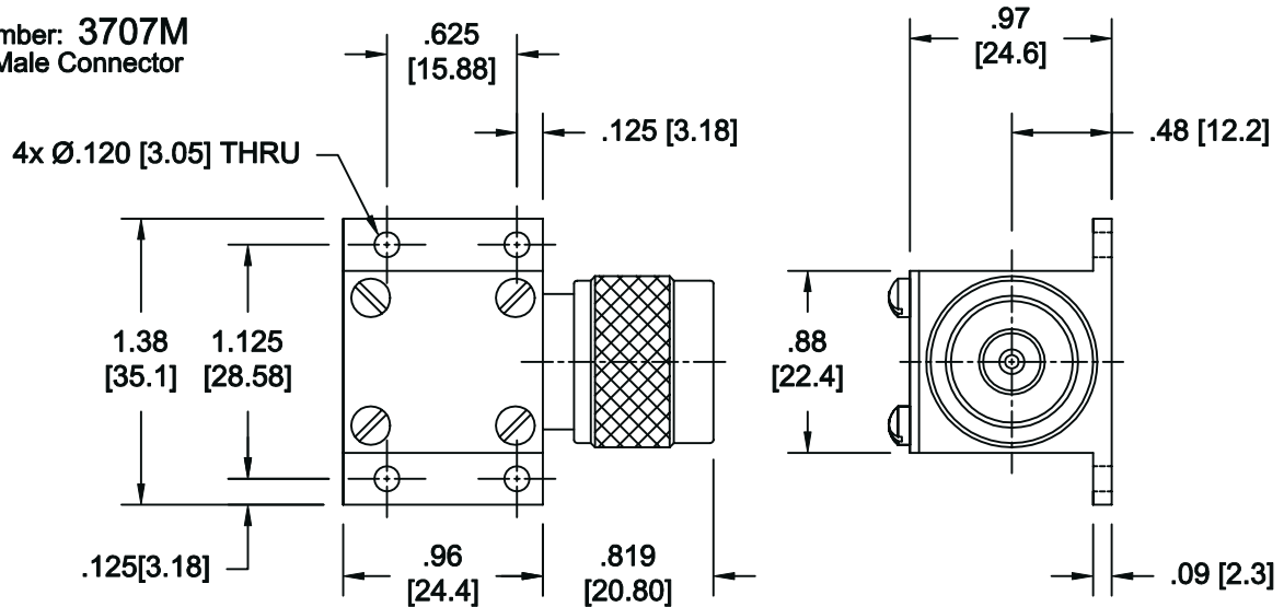
Model Number: 3707F Type N Female Connector
