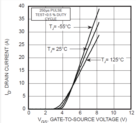
Figure 1-2. Transfer Characteristics
