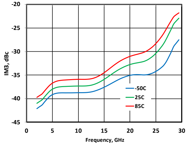
Figure 39 - IM3 vs. Temperature @ 6V/120mA, 10dBm(per tone)
