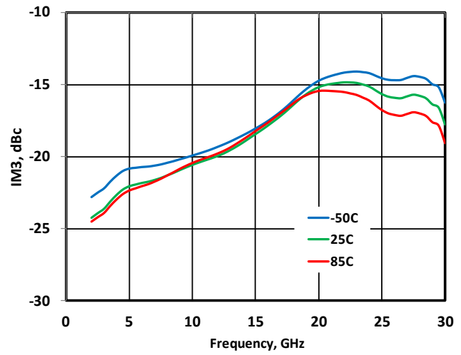
Figure 41 - IM3 vs. Temperature @ 3.5V/60mA
