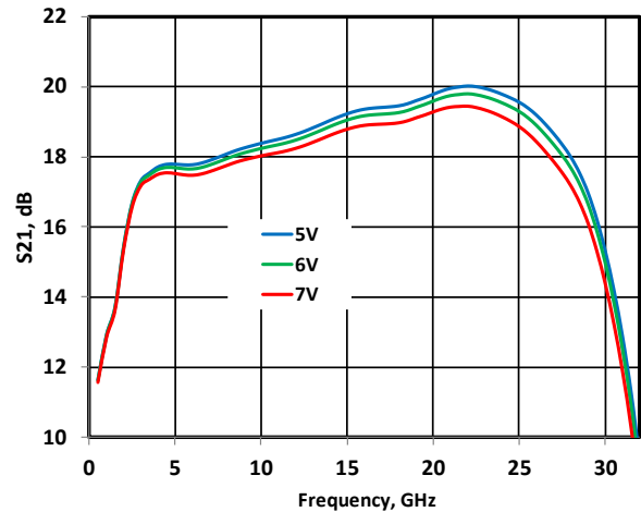
Figure 43 - Gain vs. V_{DD} @ 120mA
