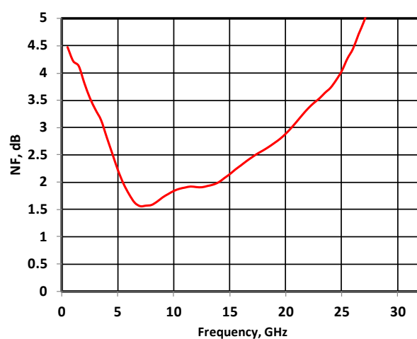
Figure 49 - NF @ 3.5V/60mA
