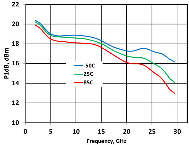
Figure 23 - P1dB vs. Temperature @ 6V/120mA
