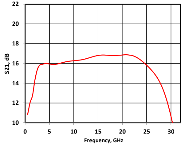
Figure 45 - Gain @ 3.5V/60mA
