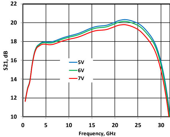
Figure 44 - Gain vs. V_{DD} @ 130mA
