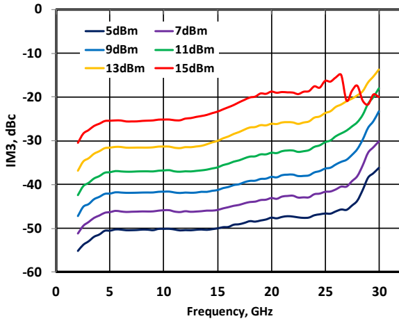
Figure 62 - IM3 vs. Power @ 7V/140mA
