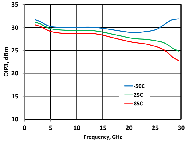
Figure 31 - OIP3 vs. Temperature @ 6V/120mA
