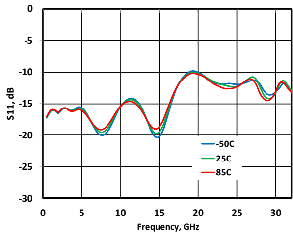
Figure 7 - S11 vs. Temperature @ 6V/120mA
