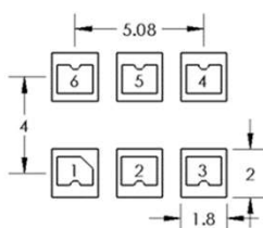
Pad Layout
