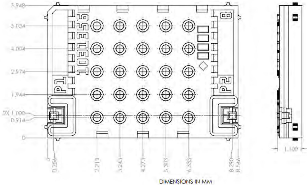
Figure 3: 2D Mechanical Drawing
