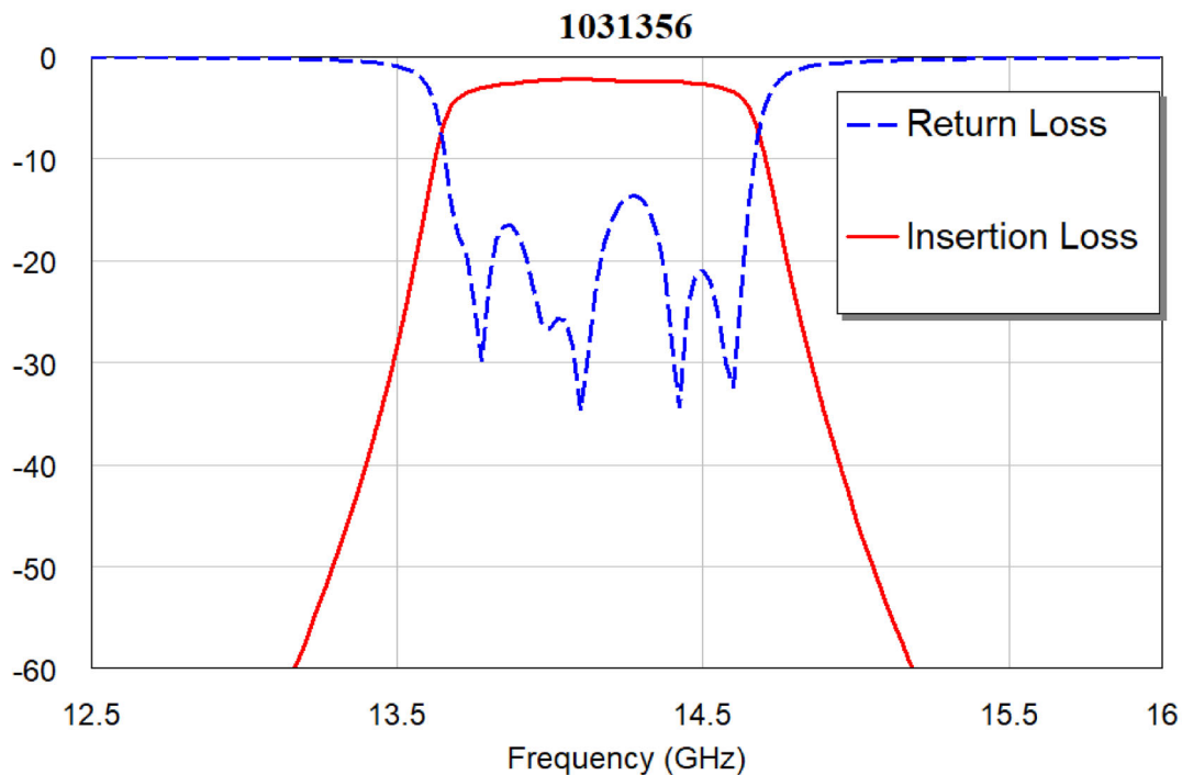
Figure 1: RF performance
