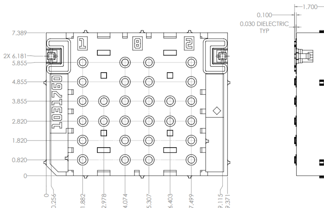
Figure 3: 2D Mechanical Drawing
