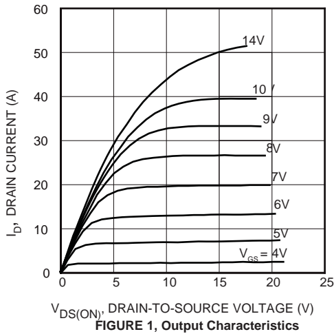
FIGURE 1, Output Characteristics
