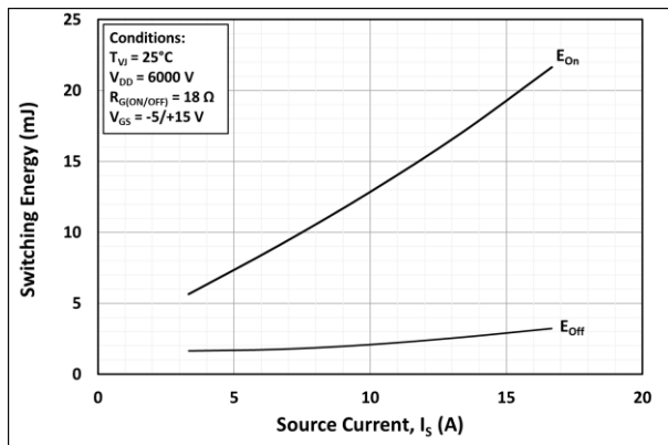
MOSFET Switching Loss at 25°C
