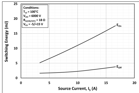
MOSFET Switching Loss at 100°C
