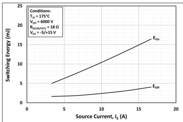
MOSFET Switching Loss at 175°C
