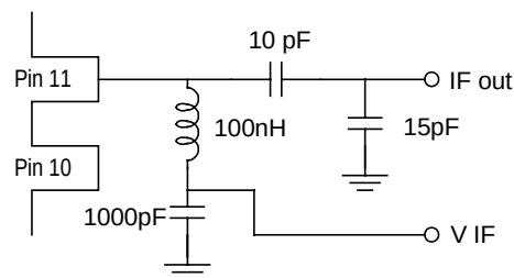
Figure 3, IF Output Match, 135 MHz
