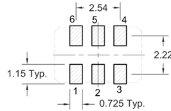
RECOMMENDED PAD LAYOUT – Top View
